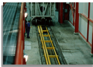
Droptable (Full Truck)
